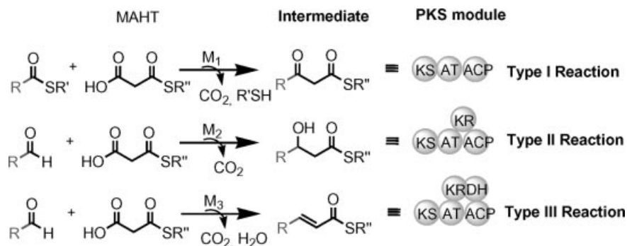
Scheme 1. Metal-catalysed reactions mimicking PKS modules.
