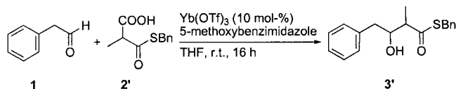
Scheme 3. Reaction between the \alpha -methyl-substituted MAHT 2' and phenylacetaldehyde ( 1 ).
