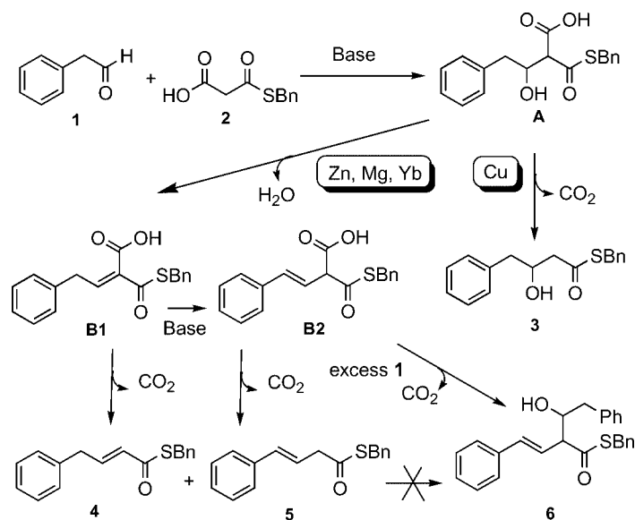
Scheme 2. Mechanistic insights into the Doebner–Knoevenagel condensations between MAHT and aldehydes.
